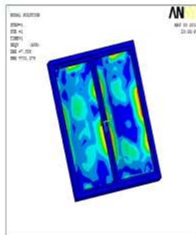
Fig.03 FEA RESULTS for pressure 1250 Pa
